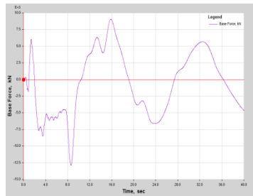
Base force (kN) for Model 1: Steel moment resisting frame
