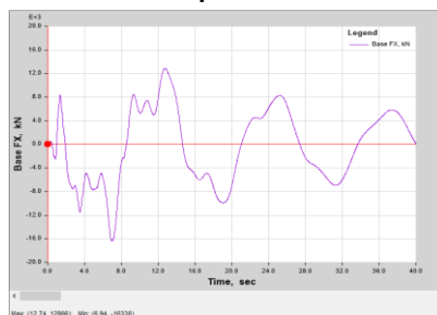
Base force (kN) for Model 2: Framed Tube Structure: Rectangular
