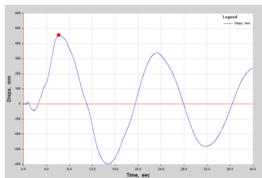
Peak displacement (mm) for Model 1: Steel moment resisting frame
