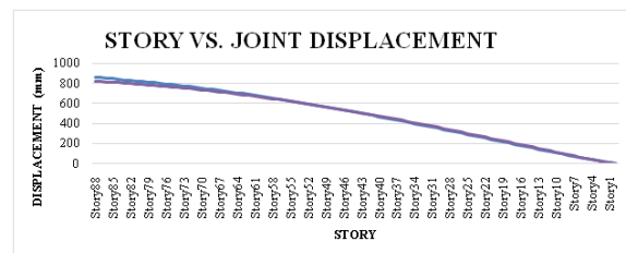
Story Displacements – Wind Analysis
