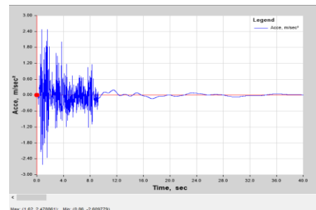
Peak acceleration (m/s 2 ) Model 2: Framed Tube
