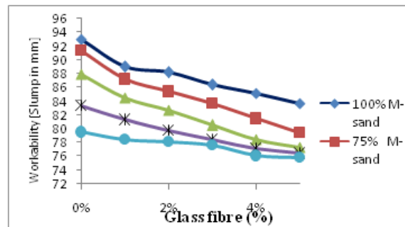
Fig. Effect of M-sand and Glass fibre on Workability of Concrete
