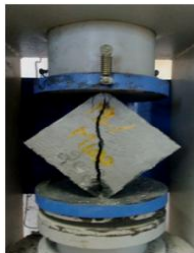
Fig. Cube after failure in split tensile test
