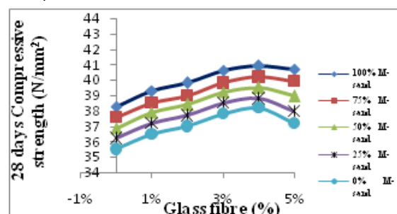
Fig. Effect of M-sand and Glass fibre on Compressive strength of Concrete when immersed in Acid[H 2 SO 4 ] for 28 days
