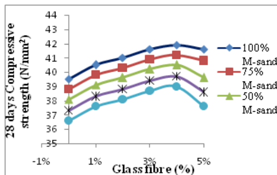
Fig. Effect of M-sand and Glass fibre on 28 days Compressive Strength of Concrete
