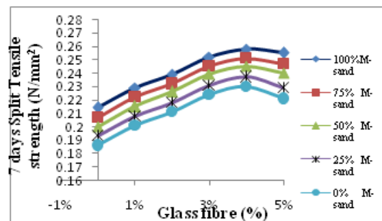
Fig. Effect of M-sand and Glass fibre on 7 days Split tensile strength of Concrete
