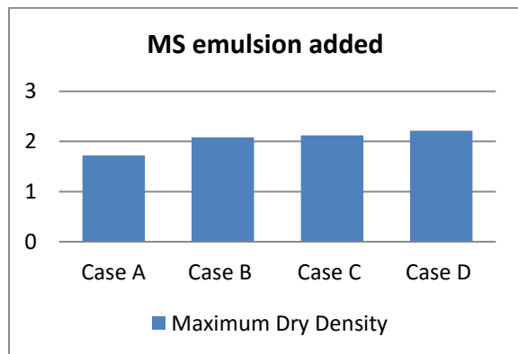
Figure 4.6 Variation of MDD for MS emulsion added. This result gives us a clear idea about used 3% bitumen content added to soil will give optimum results following mixing procedure D.
