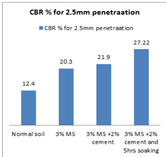
Figure 4.13 (b) Variation of CBR value for 2.5mm penetration results for MS emulsion added to soil from Case A to Case D
