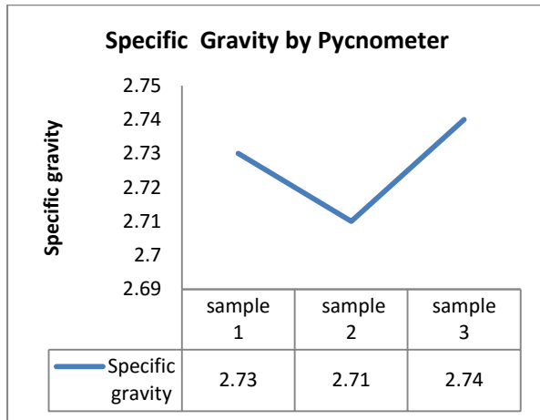
Figure 3.1(a) Specific gravity of soil samples
