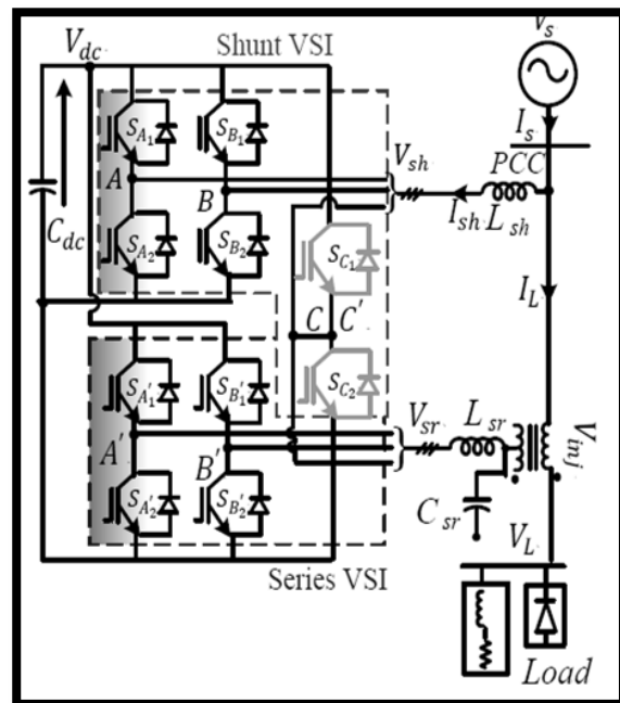
Figure 2: Proposed ten-switch UPQC.
