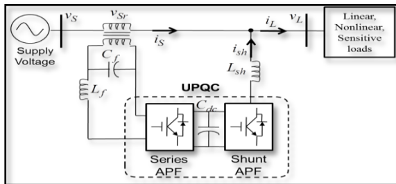
Figure 1. Conventional UPQC consist of shunt and series converters
