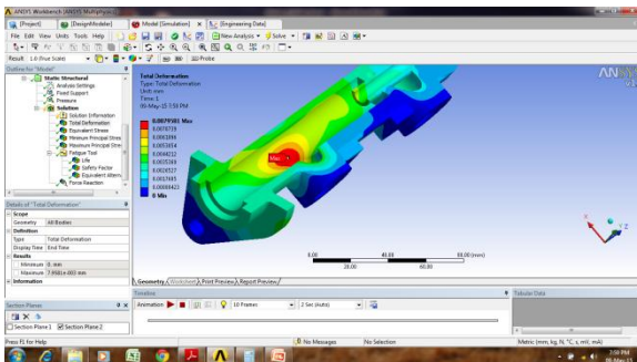
Fig: Total Deformation at the cut section
