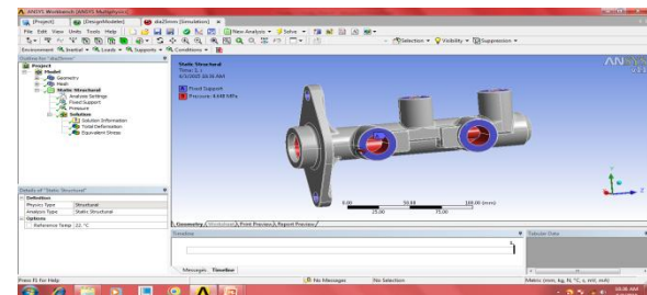
Fig: Pressure and Forced support application
