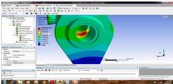
Fig: Total Deformation
