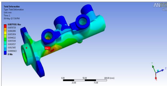
Fig: Total Deformation
