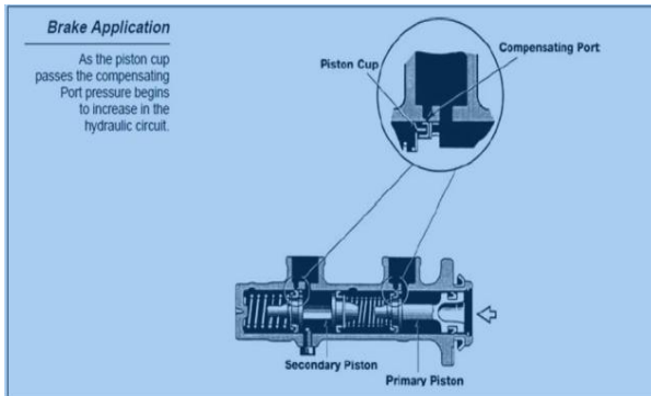
Fig:1.11 Working of master cylinder-brake application
