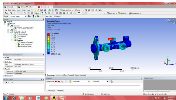
Fig: Equivalent stress
