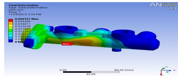
Fig: Total Deformation
