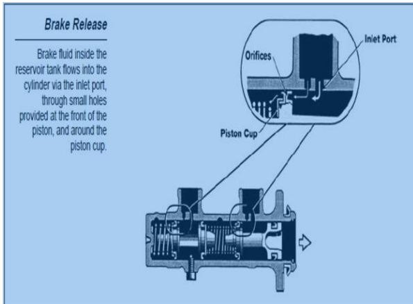
Fig: 1.12 Working of master cylinder-brake release
