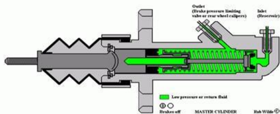
Fig: 1.6 Master cylinder
