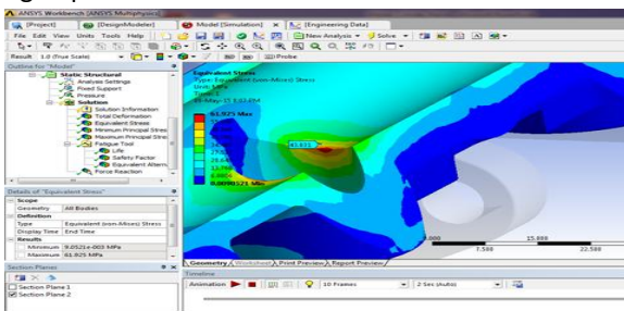
Fig: Equivalent stresses at cut section.
