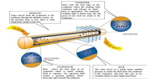
Fig. 2: Wick working phenomenon CHEMICAL INTERMEDIATE
