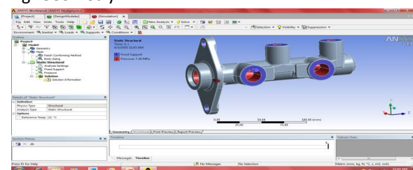
Fig: Pressure and fixed support application
