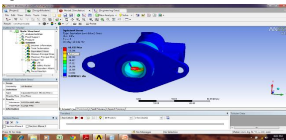
Fig: Equivalent stress
