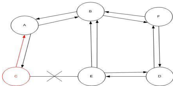
Blackhole Problem
