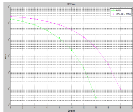
Figure 2: BER plots
